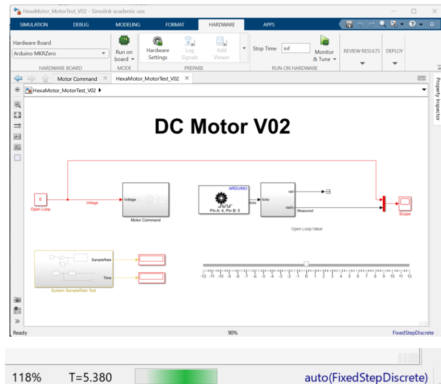
Figure 6 Simulink model for interaction with the HexaMotor Setup
